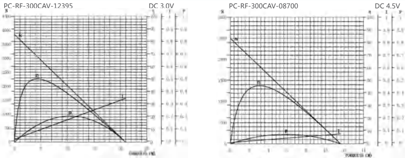
电机特性(T-N-I曲线) Motor characteristics (T-N-I curve)
