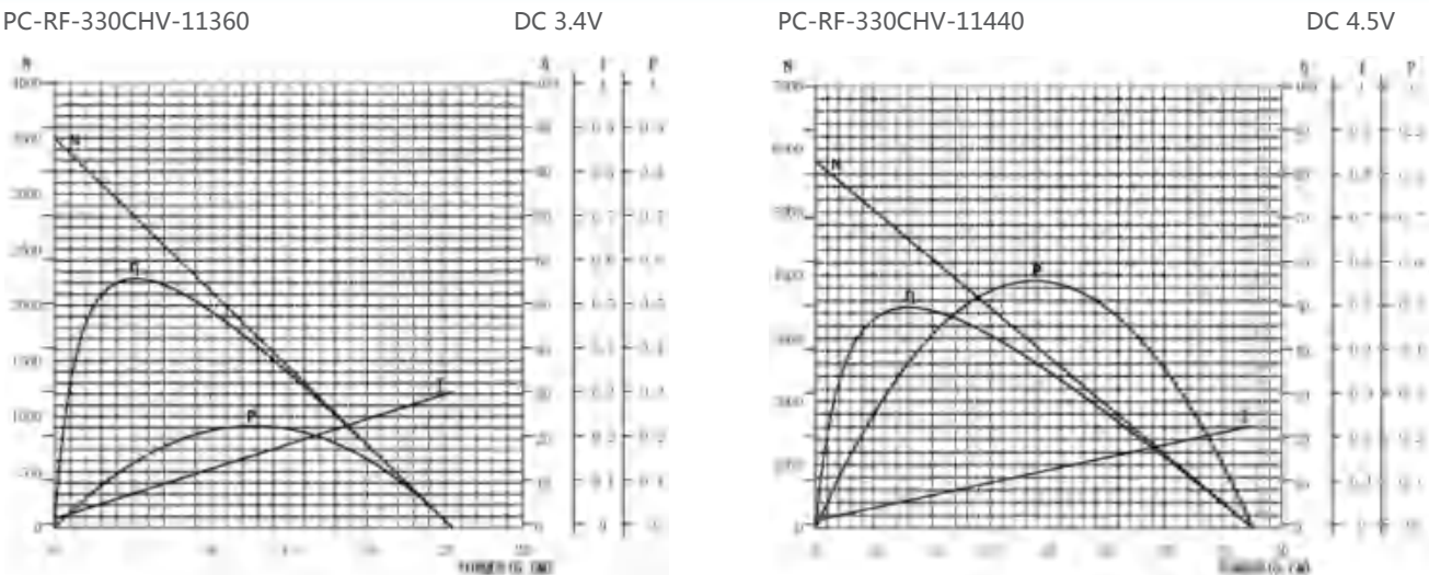
电机特性(T-N-I曲线) Motor characteristics (T-N-I curve)
